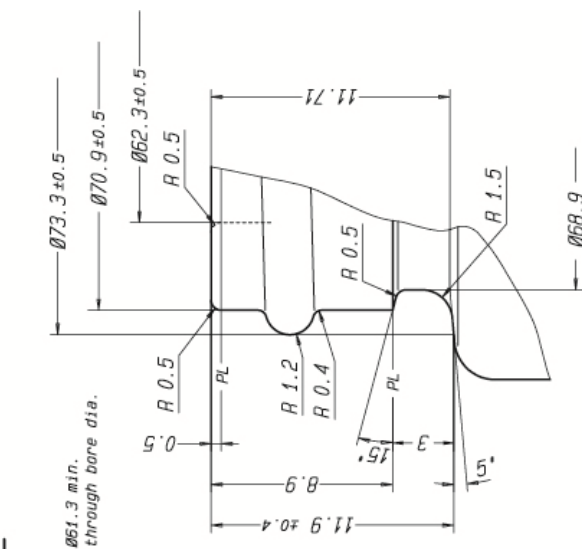
DETAIL "X" M=5/1
